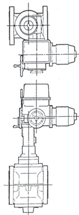
STYLE "A" (Standard mounting) MOTOR OPERATOR MOUNTED PARALLEL TO PIPE LINE
