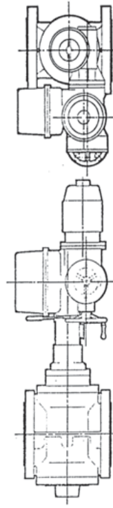
STYLE "C" MOTOR OPERATOR MOUNTED VERTICLE TO PIPE LINE
